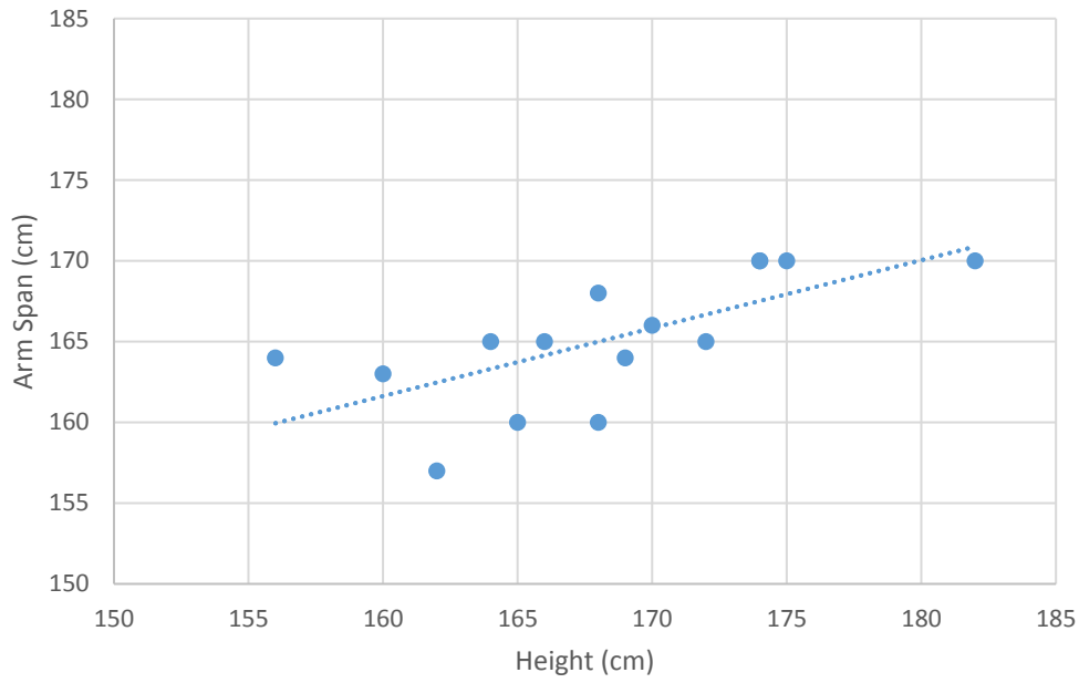
Arm Span vs. Height - Female
