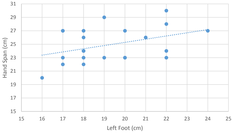
Hand Span vs. Left Foot
