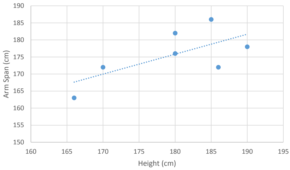
Arm Span vs. Height - Male
