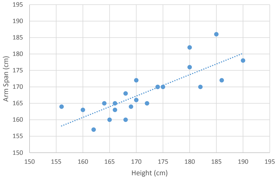
Arm Span vs. Height
